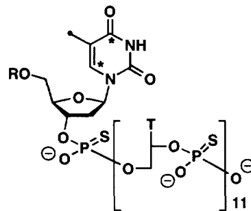
8: R = DMT; 9: R = H
