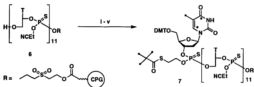
Scheme 2 i: 1a (1 equiv.)/1 H -tetrazole; ii: 1 (2 equiv.)/1 H -tetrazole; iii: sulfurization; 10 iv: 1a (5 equiv.)/1 H -tetrazole; v: sulfurization. 10
