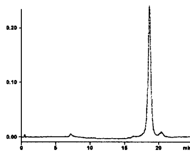
Figure 3. Ion Exchange HPLC of purified 9 . 12
